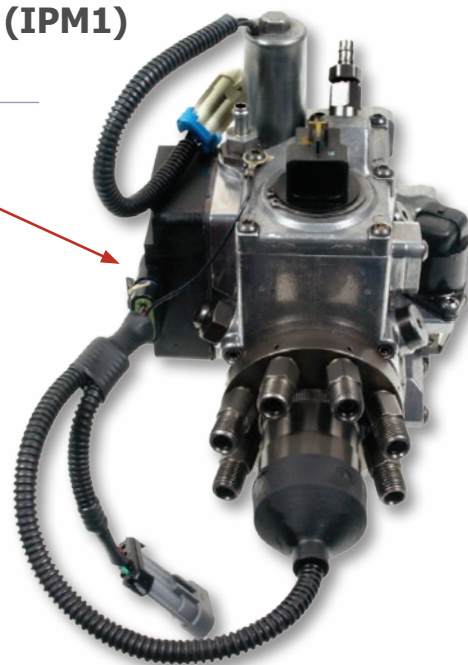
Module IP1 Injection Pump and Module Assembly
