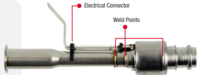
Inlet Assembly (inside of injector housing)
