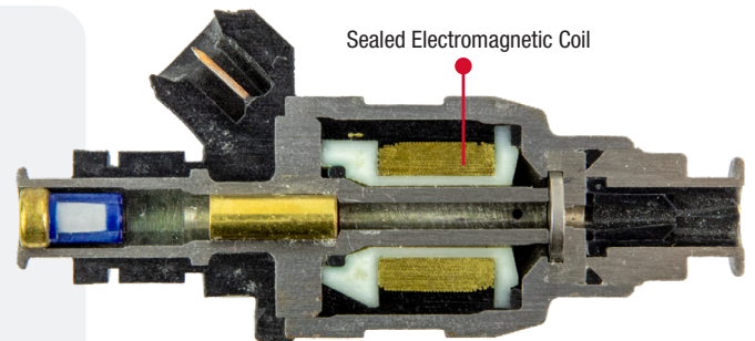
Fuel Injector Cutaway
